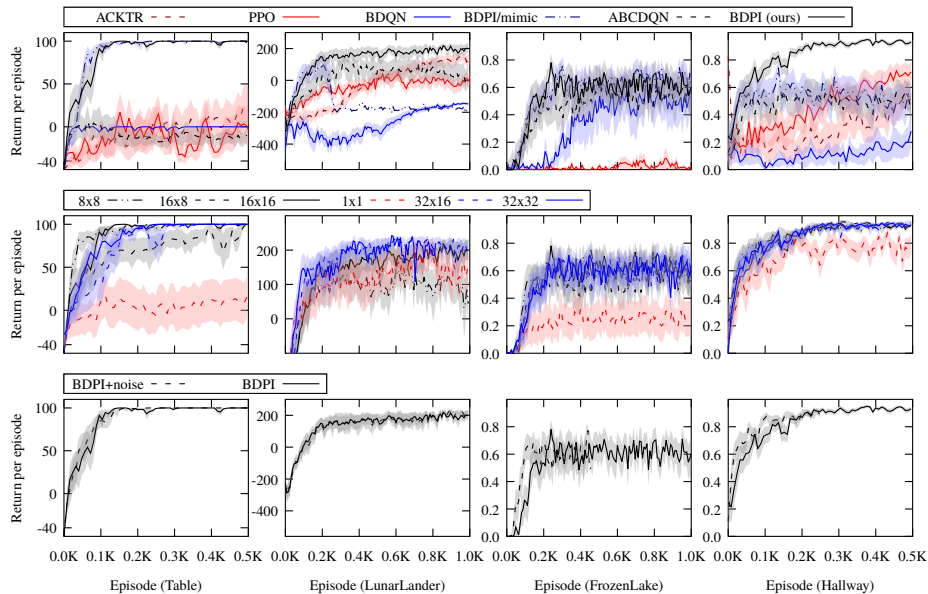
Fig. 2. Results on our four environments. Top : BDPI (16 critics, updated for 4 iterations per time-step) outperforms all the other algorithms in every environment. Middle : Varying the number of critics and how often they are trained, as long as there are more than one critic, only has minimal impact on BDPI’s performance, which demonstrates its robustness. Bottom : Adding off-policy noise (see text) does not impact BDPI on any of the environments.
